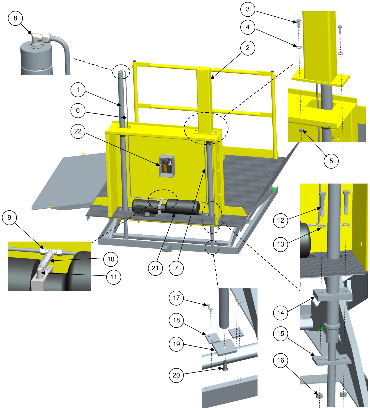
FIGURE #21 – Surface Mount Dock Lift Hydraulics
